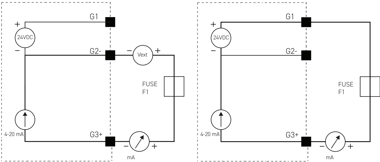
AC ACTIVE AND PASSIVE 4-20 mA OUTPUT CONNECTION
