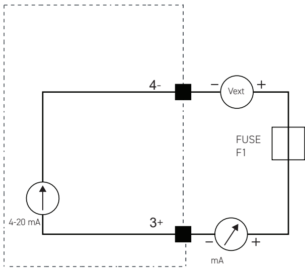
PASSIVE 4-20 mA OUTPUT CONNECTION
