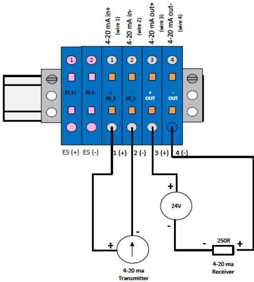
4-20mA INPUT PASSIVE 4-20mA OUTPUT
